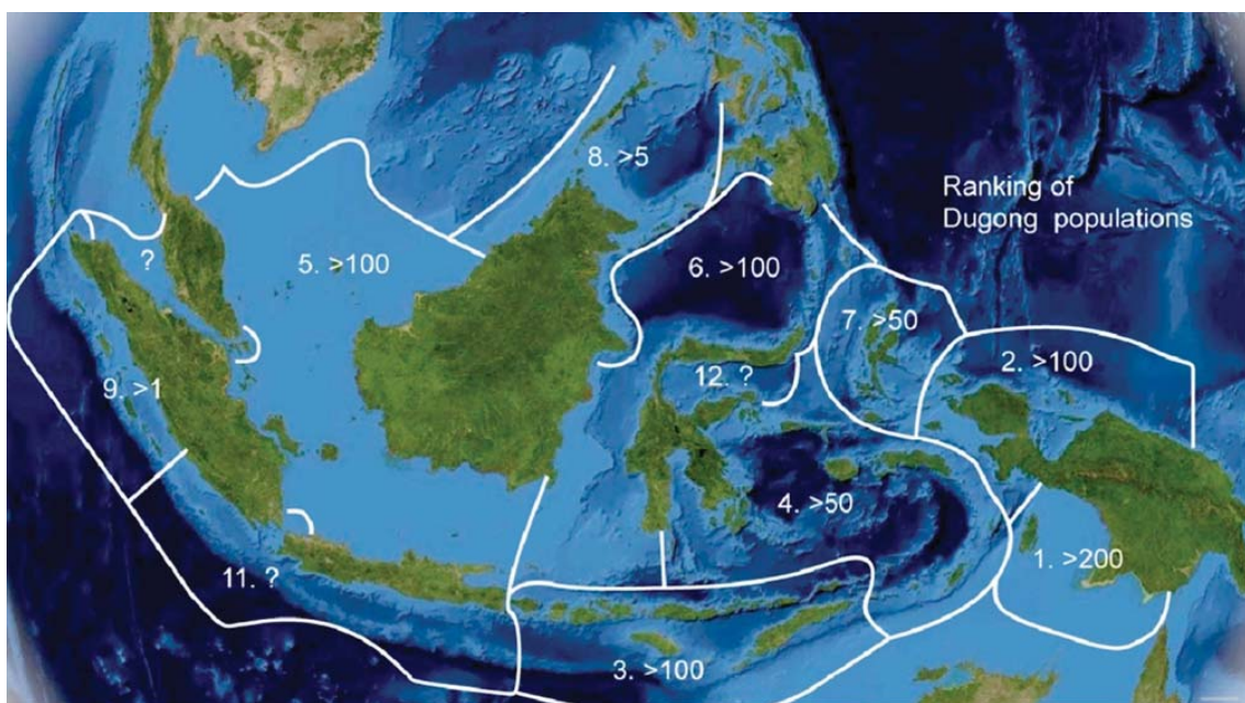
Figure 19. Estimated size of Dugong populations across Indonesian ecoregions, with a ranking of ecoregion importance for Dugongs. (S. Campbell)
